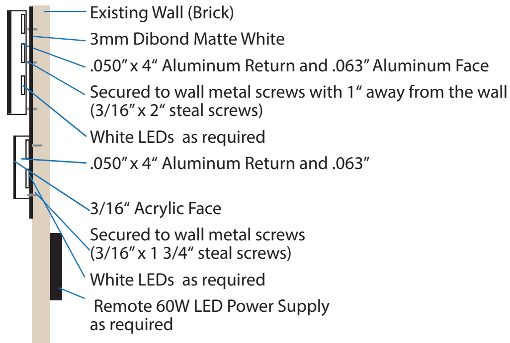
Side View (Halo illuminated Letters and cabinet)
